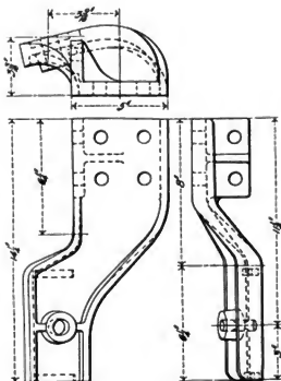
Figs. 3879-3881. Uncoupling Chain Sheave Hanger.
